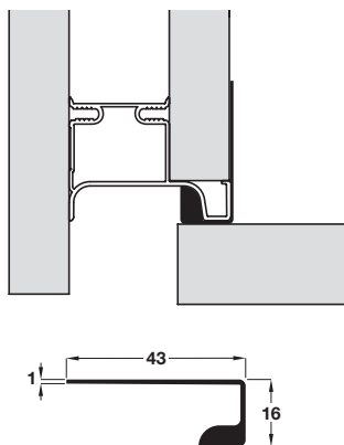
GOLA System D profile, for vertical fixing between cabinet and oven
