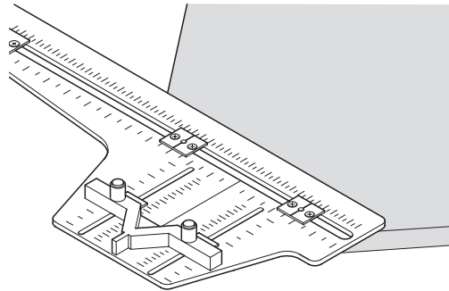
For drilling on flaps at 45° angle
