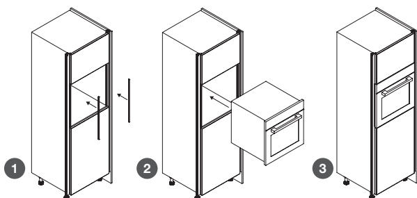
GOLA System E profile, for vertical fixing between cabinet and oven
