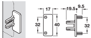
Dowel fixing
