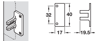
Screw fixing
