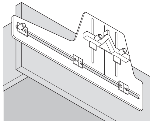
For drilling on panels
